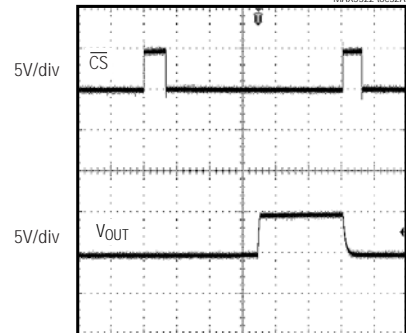
UNIPOLAR SOFTWARE-SHUTDOWN RESPONSE
