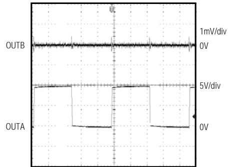
DAC-TO-DAC CROSSTALK
