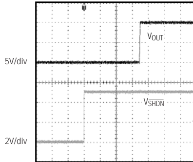
BIPOLAR RELEASE FROM HARDWARE SHUTDOWN RESPONSE
