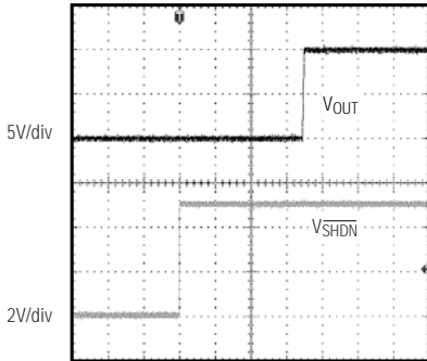
UNIPOLAR RELEASE FROM HARDWARE SHUTDOWN RESPONSE
